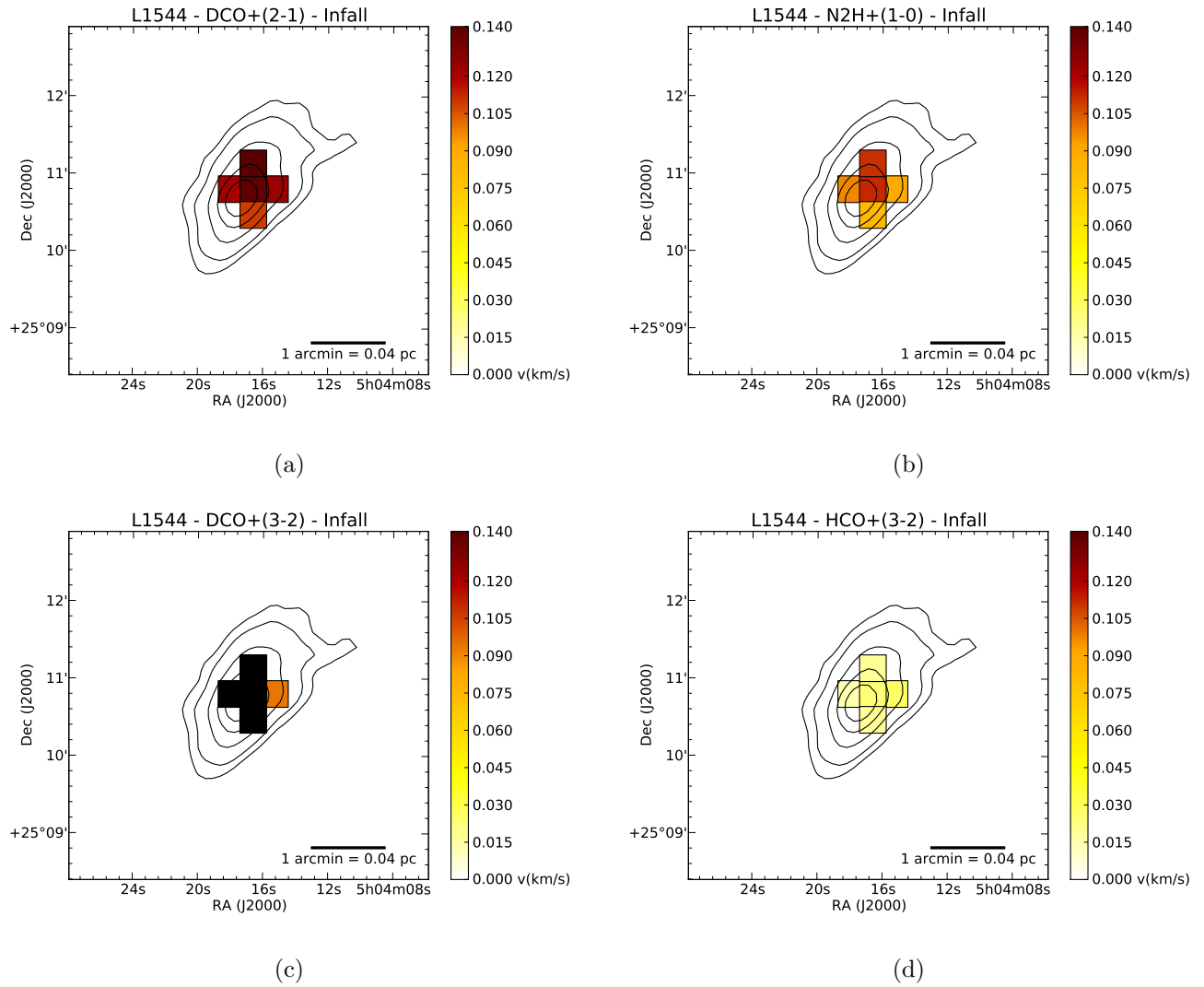
Fig. 8.—: Infall/outflow velocity gradient maps for L1544 with velocities below three times their corresponding error represented by black.
