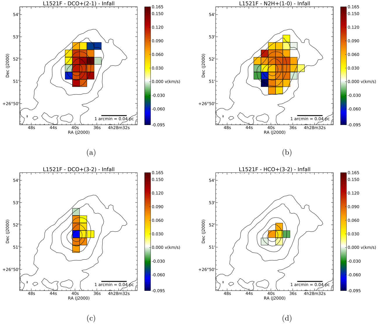
Fig. 7.— Same as Figure 5, for the core L1521F. Note that all four velocity scale bars are uniform. Outflows can be seen most apparently in the lower left and upper right corners of (a) and (b), which matches the bipolar outflow discovery of Takahashi et al. (2013).
