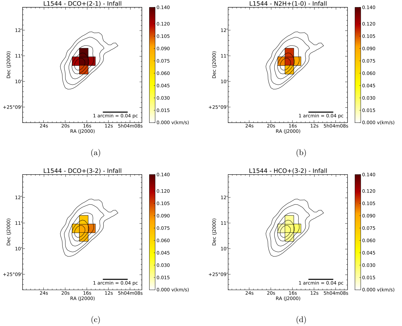
Fig. 5.—: Infall/outflow velocity gradient maps for L1544 in (a) \text{DCO}^+(2-1) (b) \text{N}_2\text{H}^+(1-0) (c) \text{DCO}^+(3-2) and (d) \text{HCO}^+(3-2) . Velocities are in \text{km s}^{-1} . Background contours are the same as in Figure 3a. Note that all four velocity scale bars are uniform.
